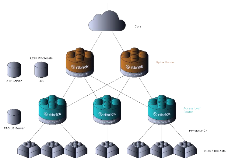
Spine-Leaf BNG
