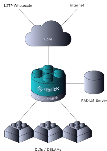
Consolidated BNG
