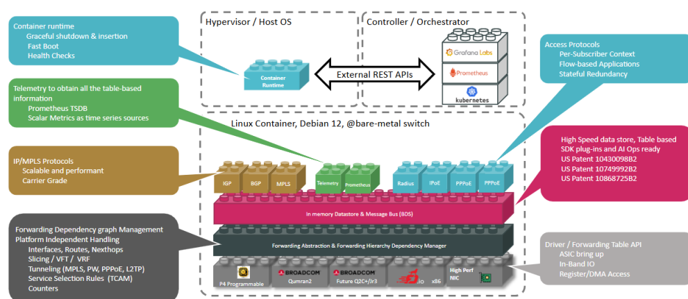
Figure 1. RBFS Overview
