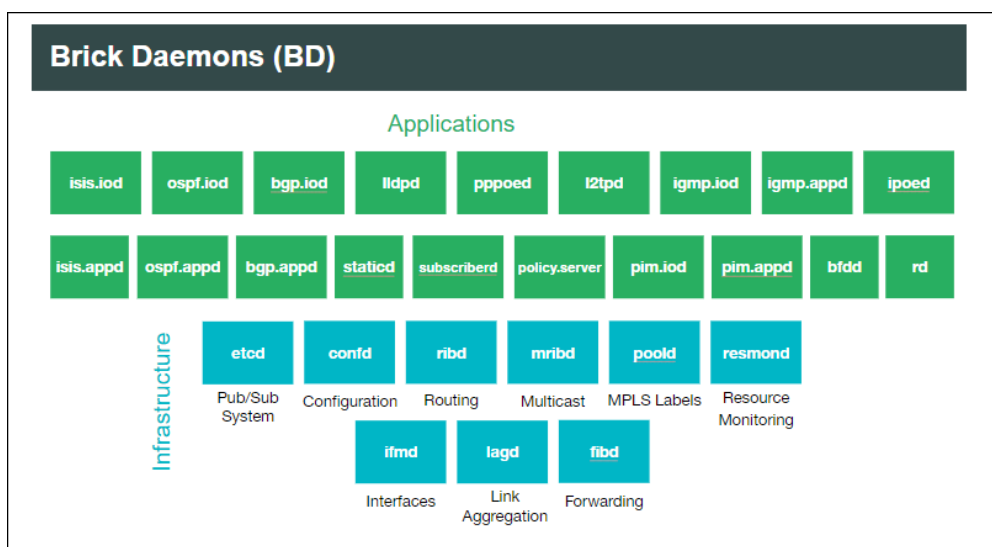
Figure 2. RBFS Microservices
