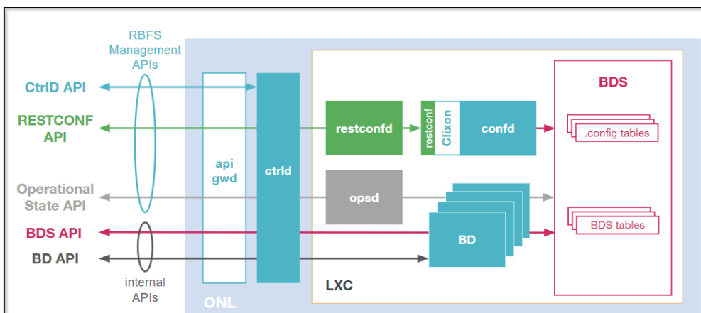
Figure 3. RBFS API Overview
