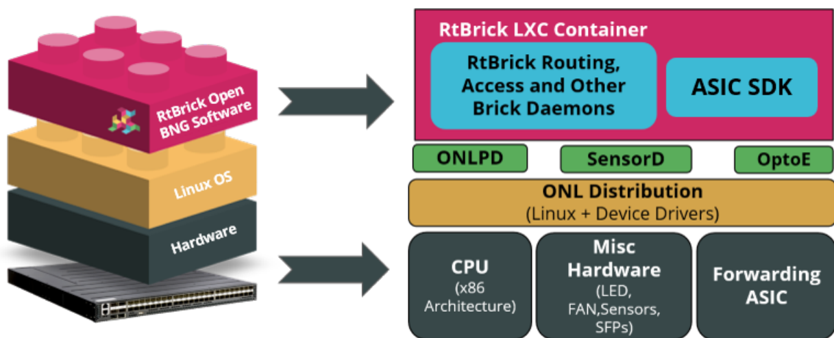
Figure 4. Platform Overview
