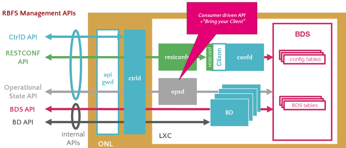
Figure 1. RBFS REST APIs
