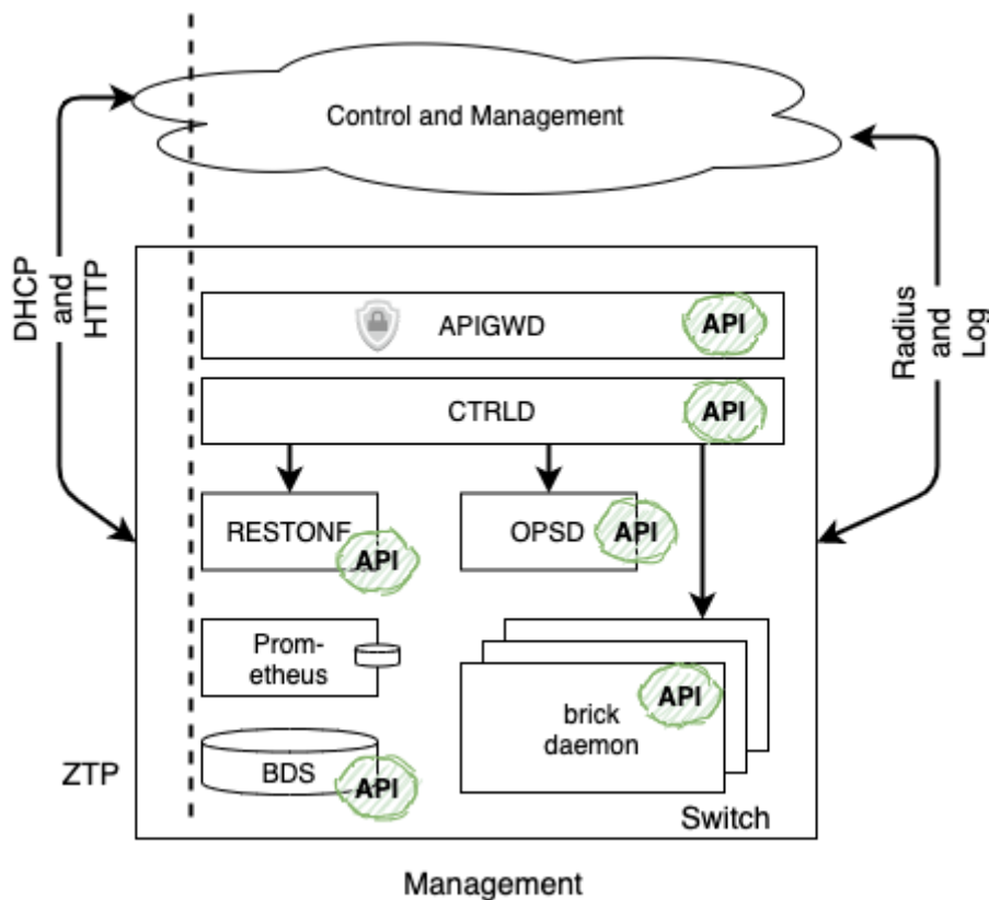
Figure 2. CtrlD Overview
