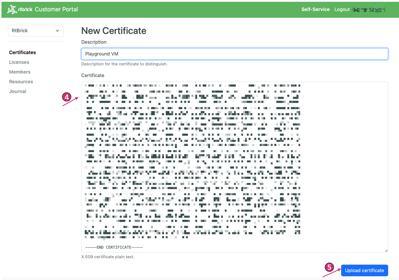
Figure 4. Client Certificate Upload Form
