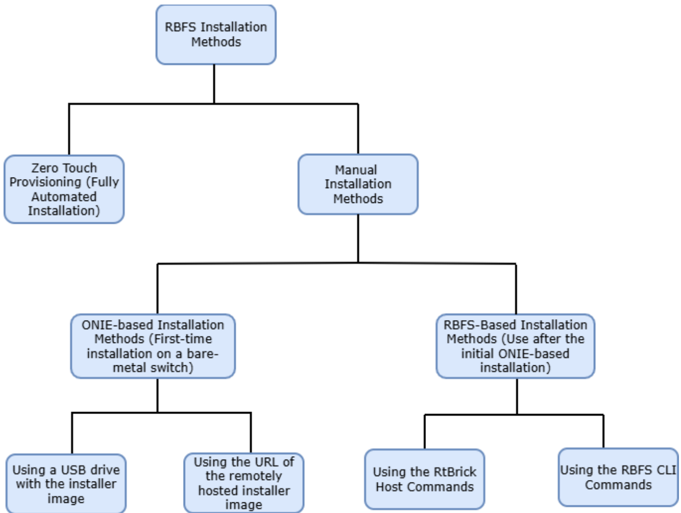
Figure 1. RBFS Installation methods high level view
