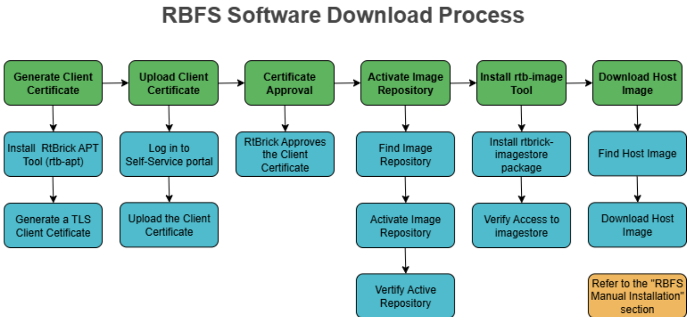
Figure 2. RBFS Software Download Process
