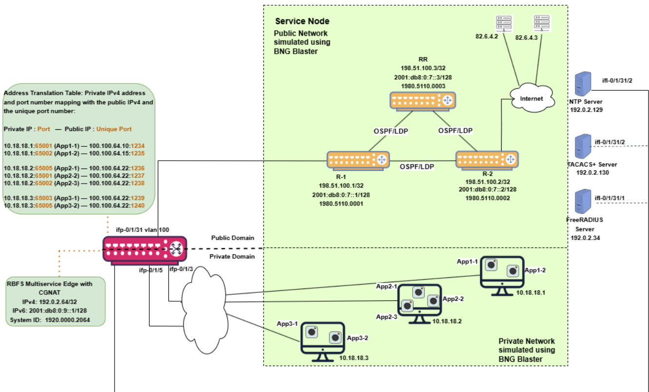
Figure 11. RBFS Multiservice Edge with CGNAT Implementation
