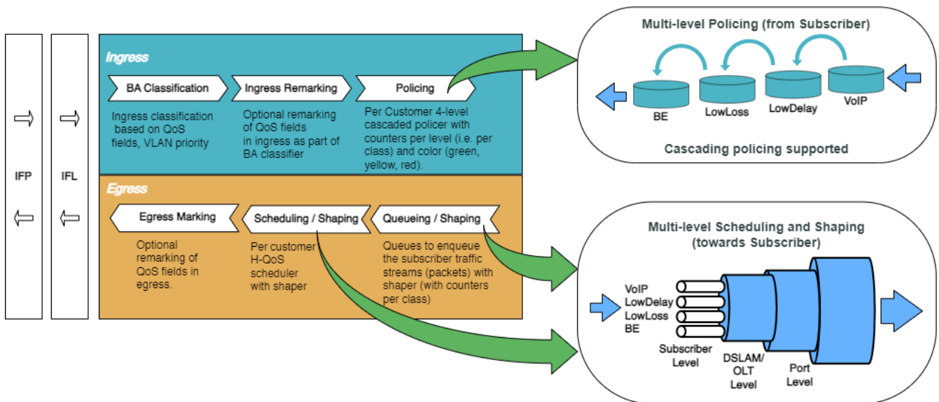
Figure 16. Hierarchical Quality of Service primitives
