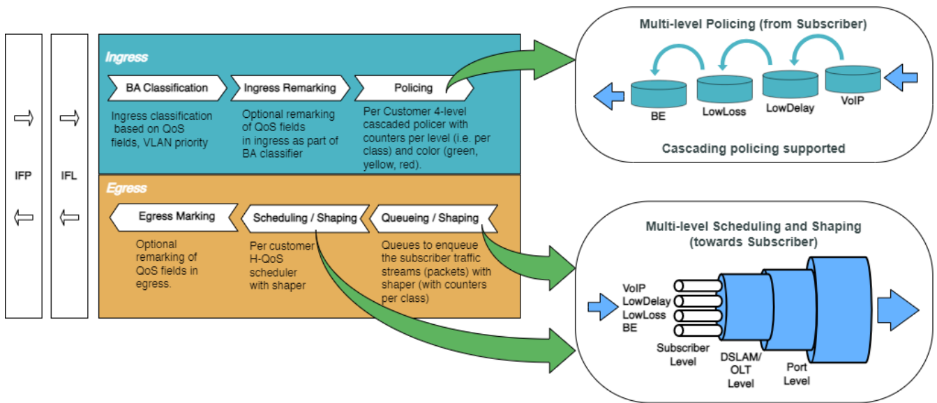
Figure 3. Hierarchical Quality of Service Primitives
