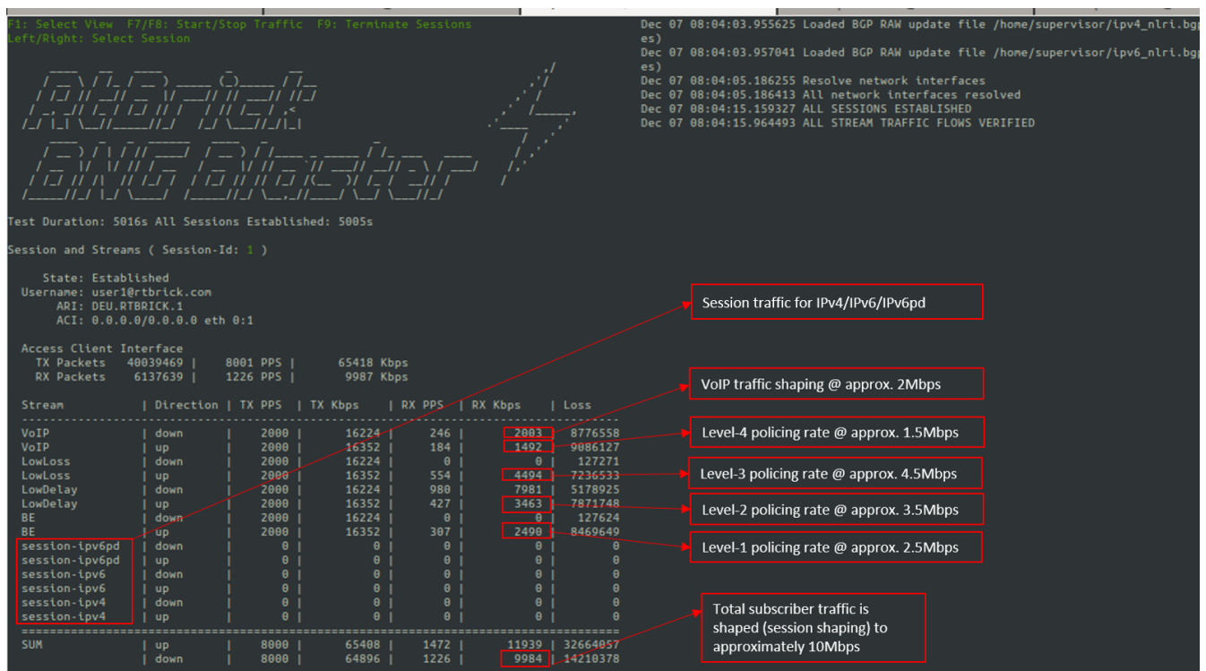
Figure 10. Reading Output from BNG Blaster
