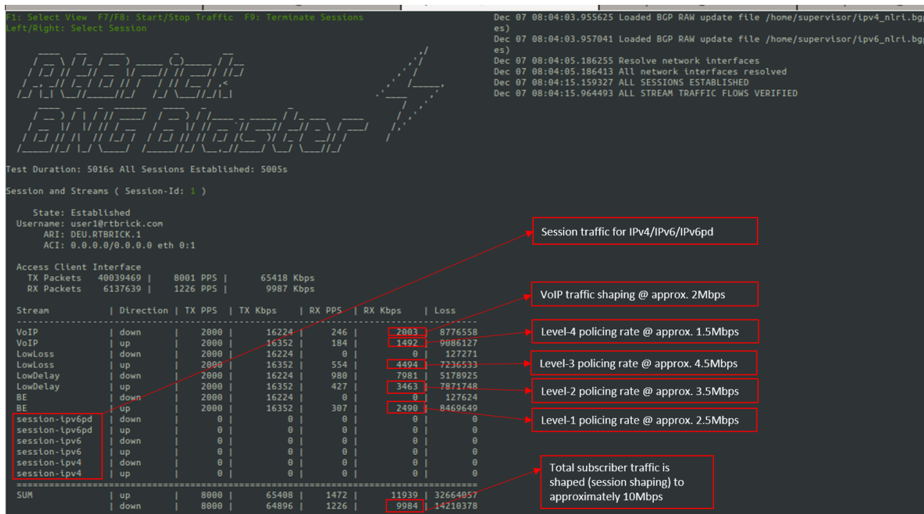
Figure 5. Reading output from BNG Blaster
