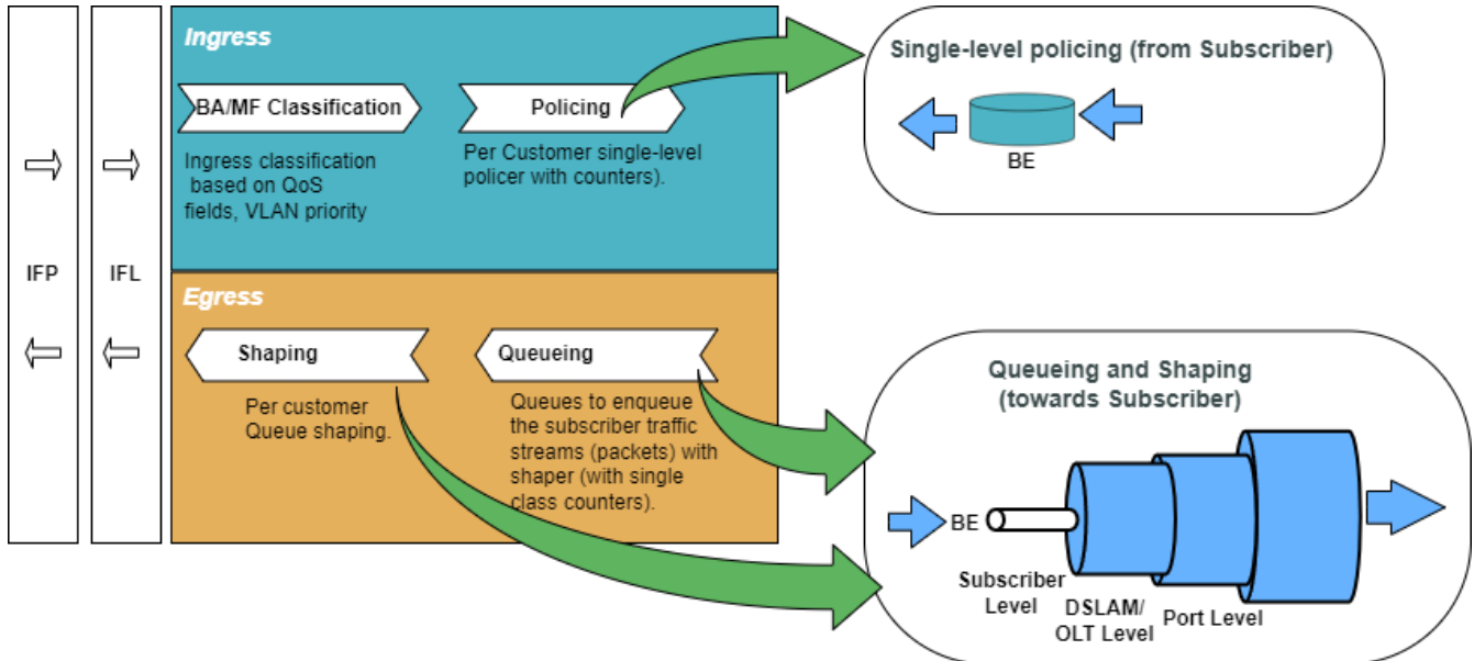
Figure 13. QoS Configuration for Ingress and Egress Traffic
