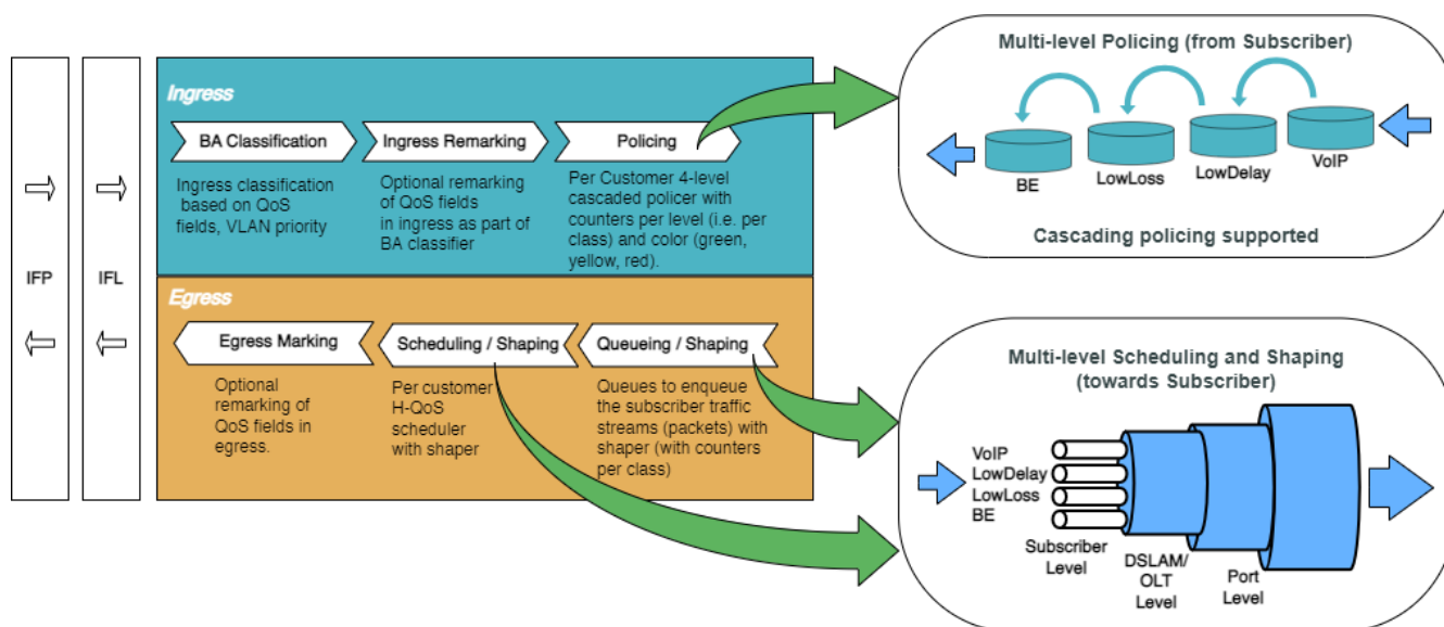
Figure 8. Hierarchical Quality of Service Primitives
